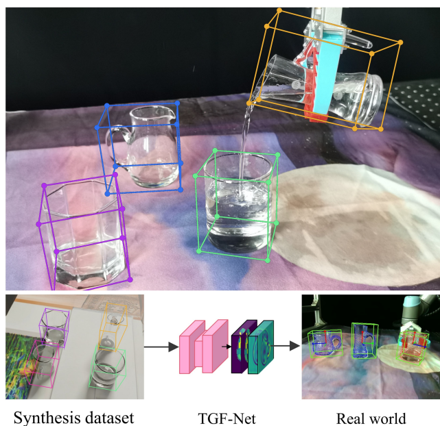
Fig. 1. TGF-Net is trained entirely using synthetic datasets and infers accurate 6D poses of transparent objects from monocular RGB images. The estimated 6D pose can be directly used for downstream manipulation tasks of the robot (e.g. grasping and pouring).
