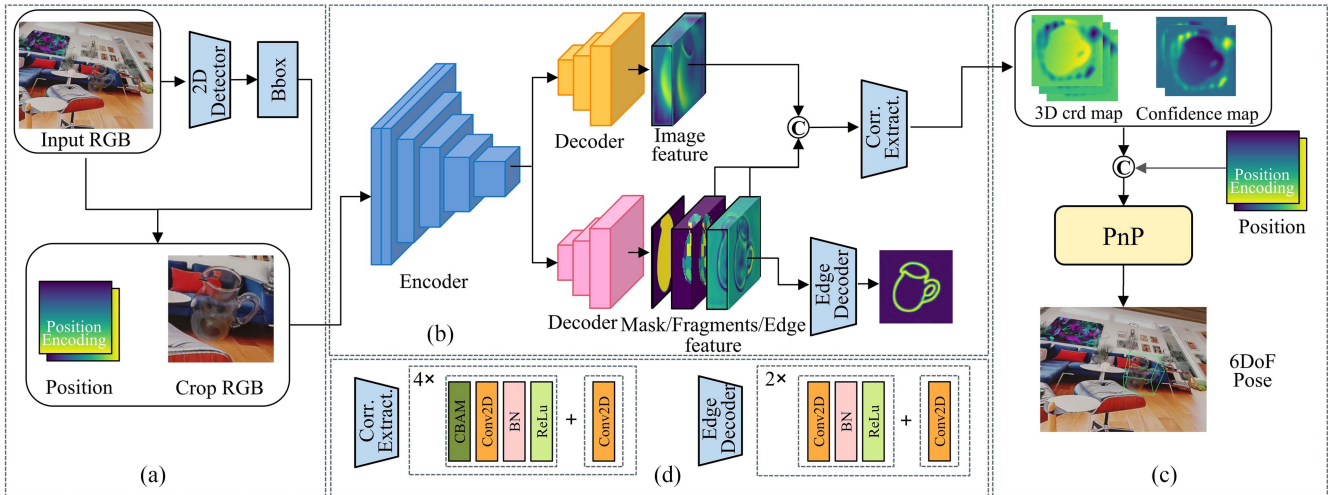
Fig. 3. Overview of our network. Our network consists of three building blocks: (a) Object detection and image enhancement. (b) The main structure of the network. After the input image is encoded and decoded, a regular flow and a geometric flow are formed, and the correspondence is extracted by fusion between the two flows. (c) A learnable PnP network for 6D pose estimation. (d) The detailed structure of part of the network, where CBAM means convolutional block attention module [43].
