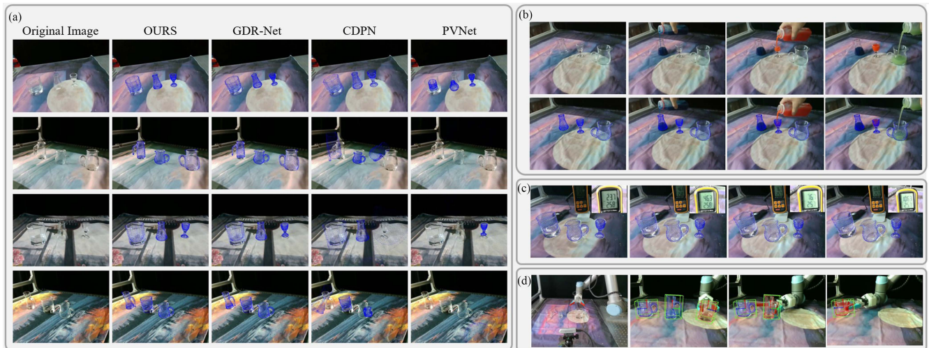
Fig. 5. Qualitative results in real scenarios. Each object point cloud is transformed with the estimated pose and then projected to the 2D image. (a) Real-world experiments in different background. We compare TGF-Net with GDR-Net, CDPN and PVNet under the same conditions. (b) The 6D pose estimation of transparent objects with different colored internal liquids. (c) The 6D pose estimation of transparent objects under different illumination conditions. (d) Transparent objects grasping experiment. The robotic arm grasps the transparent object according to the 6D pose, and the red point cloud projection indicates the selected object to be grasped.
